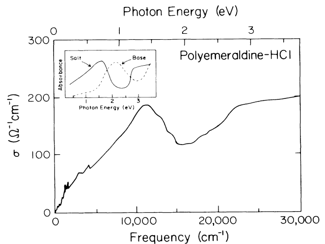
FIG. 2. Optical absorption spectra of protonated polyemeraldine. Inset: Near-ir and visible absorption for both emeraldine base (insulating) and emeraldine salt (metallic) forms.
